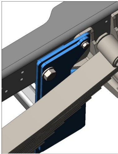
Figure 9: Front mounting plate installation
